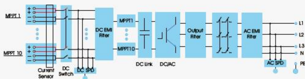
Topology Diagram
